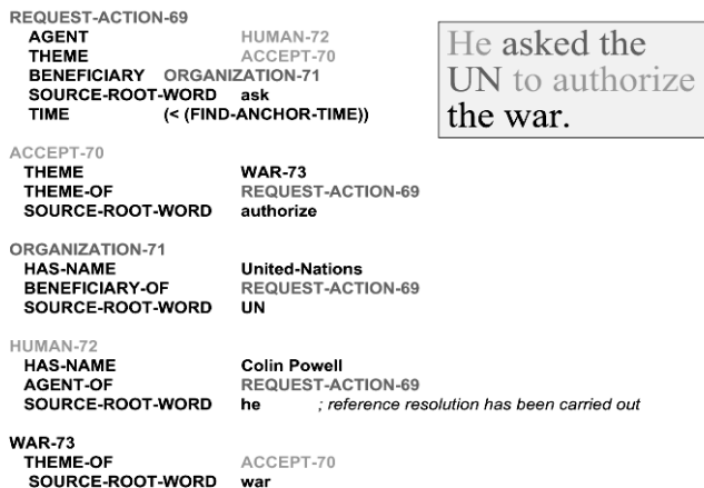
Figure 3. OntoSem constructs this text meaning representation (TMR) for the sentence “He (Colin Powell) asked the UN to authorize the war.”
