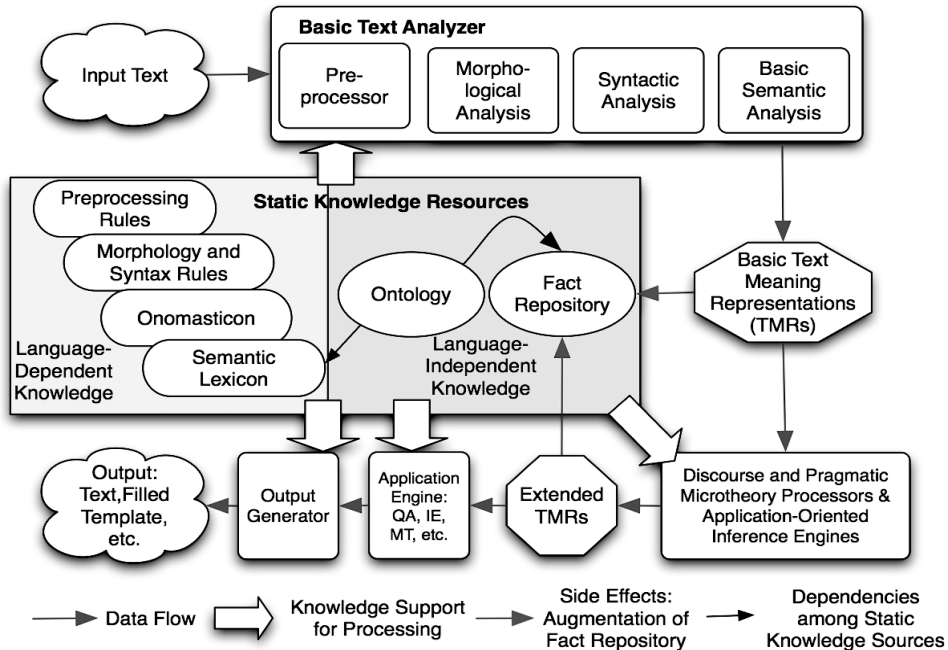
Figure 1. OntoSem is a large scale, sophisticated natural language understanding system that uses a custom frame-based knowledge representation system with an extensive ontology and lexicon.
